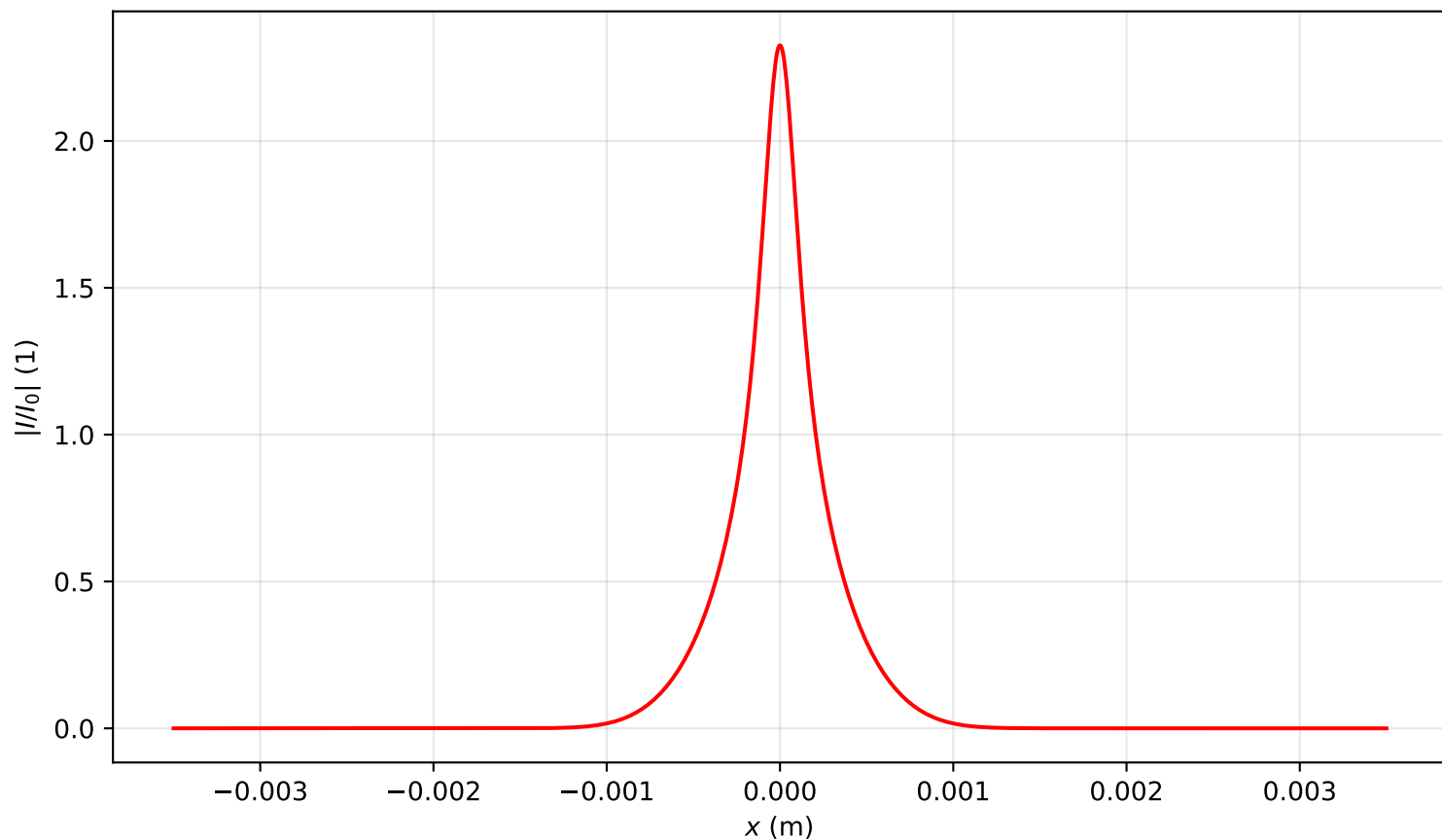
Intensity profile I(x, y = 0, z = 0.239)/I_0 , P_{in}=9.0P_{cr} , artificial time
